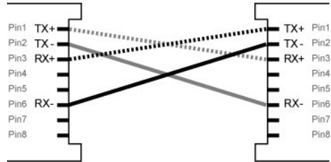
The standard cable, RJ-45 pin placement
